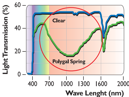
— Spectral transmission of Thermogal 32 mm - Clear — Spectral transmission of Thermogal 32 mm - Polygal Spring
