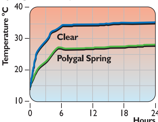
— Thermogal 32 mm - Clear temperature increase — Thermogal 32 mm - Polygal Spring temperature increase
