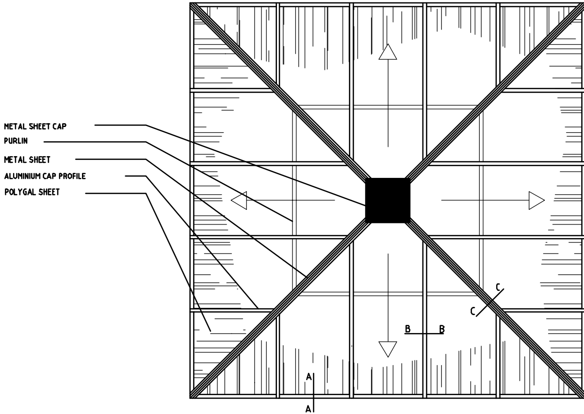
PYRAMID PLAN
